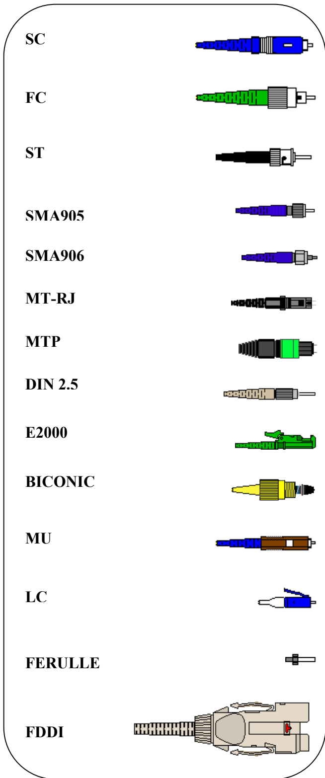
Connector Types
